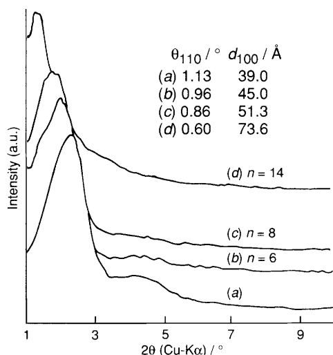
Fig. 1 X-Ray diffraction patterns of mesoporous silica formed with a cationic surfactant (a) in the absence of a solubilizing agent and (b)–(d) in the presence of normal alkanes, C_nH_{2n+2} (with 1:1 molar ratio of the surfactant and the alkane). The n values are indicated beside the diffraction profiles.
