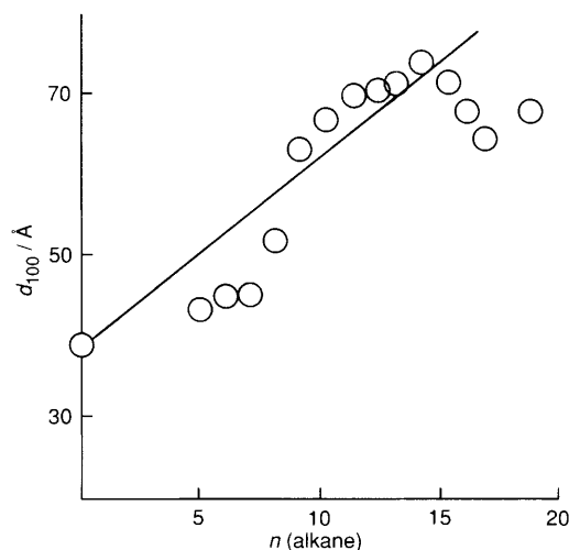
Fig. 3 Plot of the observed d_{100} values of mesoporous silica against the number of carbon atoms, n , of the alkane. The straight line is that expected if the lengths of the alkane chain and surfactant tail were to be additive in forming the micelle template for the formation of mesoporous silica.
