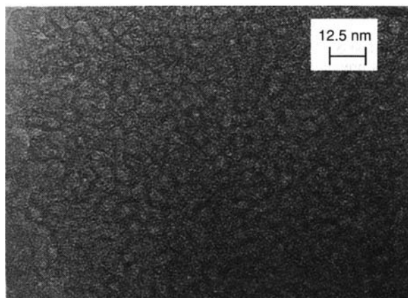
Fig. 4 TEM image of mesoporous silica obtained by using n\text{-C}_{10}\text{H}_{22} as the solubilizing agent. The pore size is ca. 66 \text{ \AA} .
